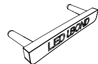
Endcap Art no.: 51008-D49 16 (3.3) x 40 x 6 mm
